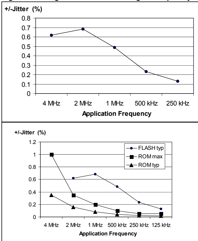
Figure 77. Integrated PLL Jitter vs signal frequency 1
