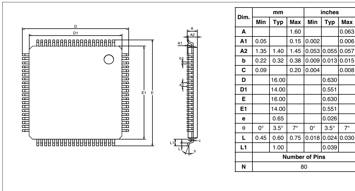
Figure 98. 80-Pin Low Profile Quad Flat Package
