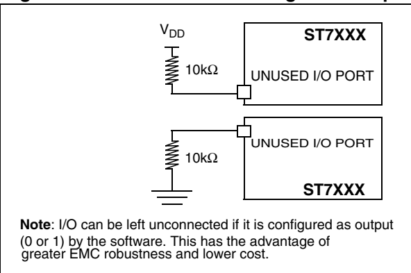
Figure 78. Unused I/O Pins configured as input
